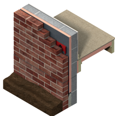
Full and partial fill cavity wall insulation
